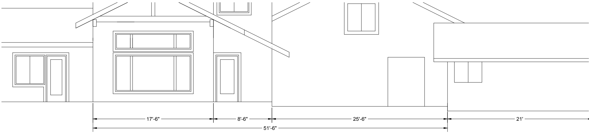
East Elevation
