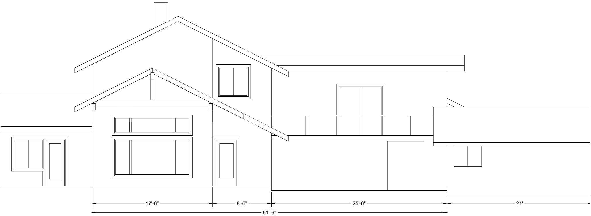
East Elevation
