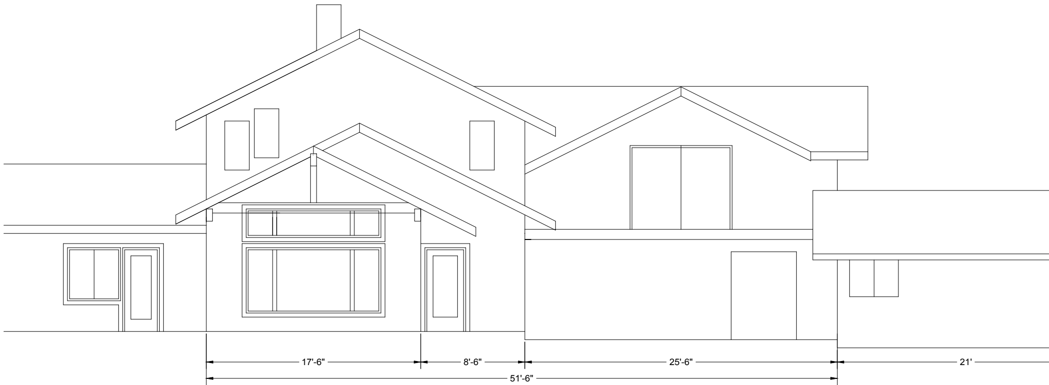
East Elevation
