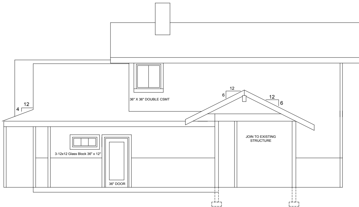
South Elevation
