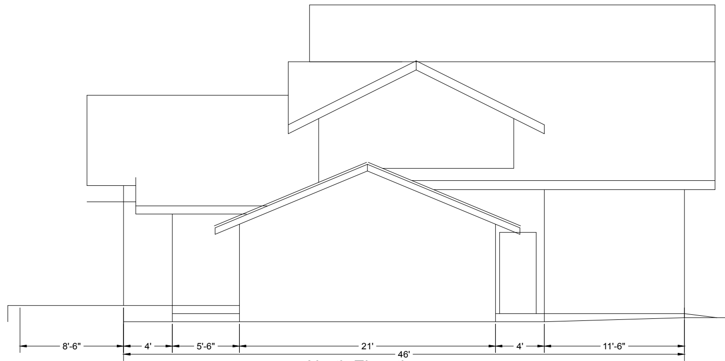
North Elevation
