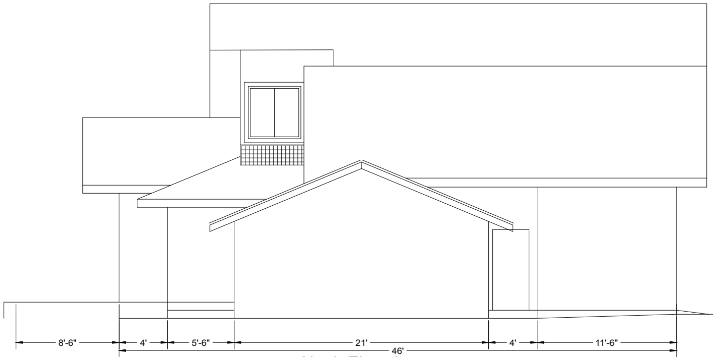
North Elevation
