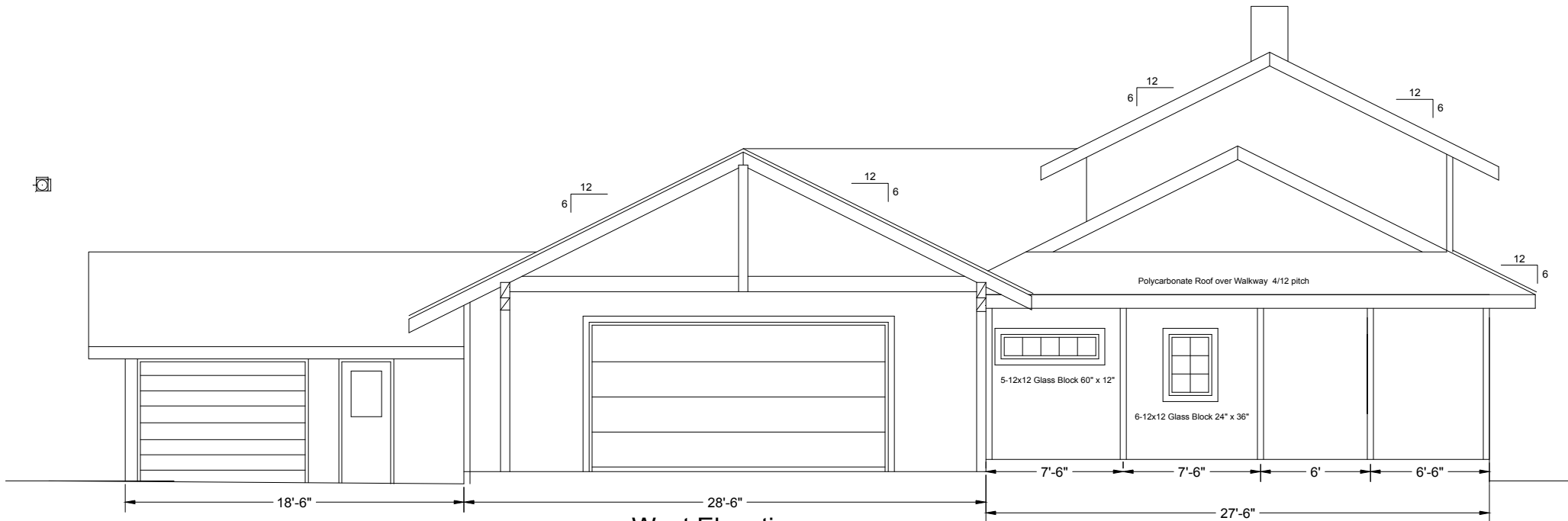
West Elevation
