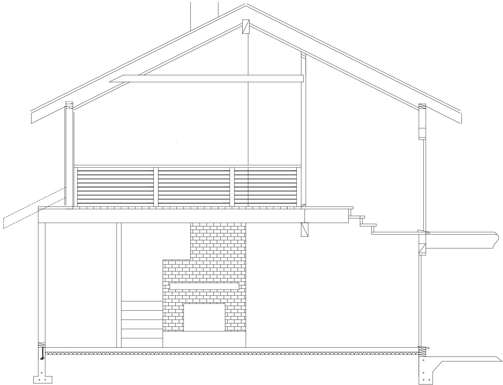
X-SECTION S-N-4
