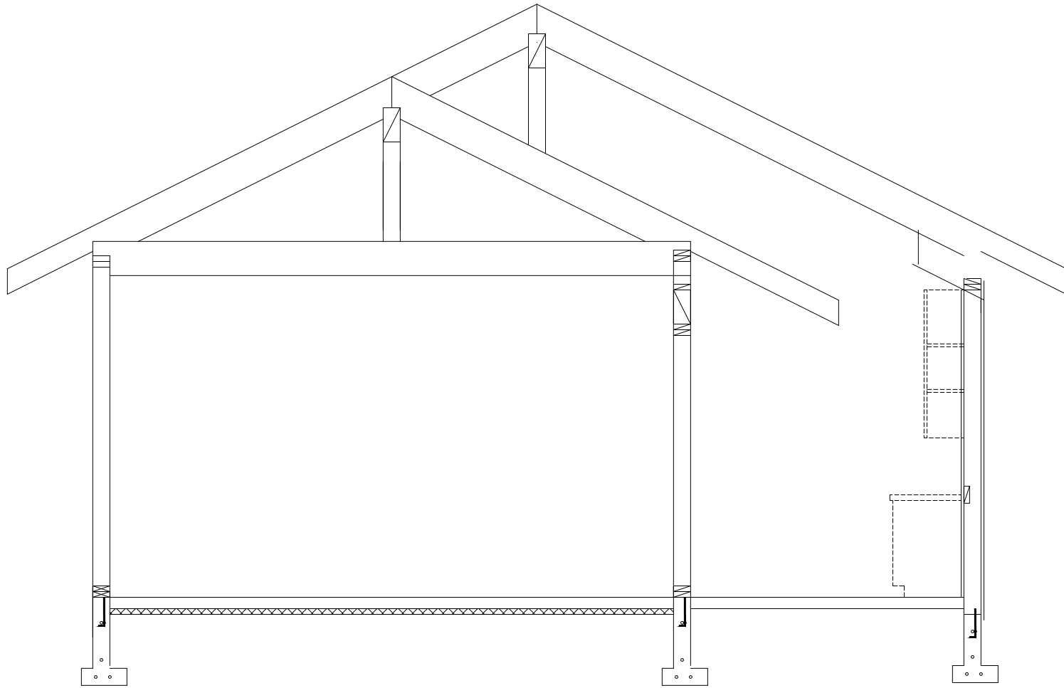
X-SECTION S-N-1
