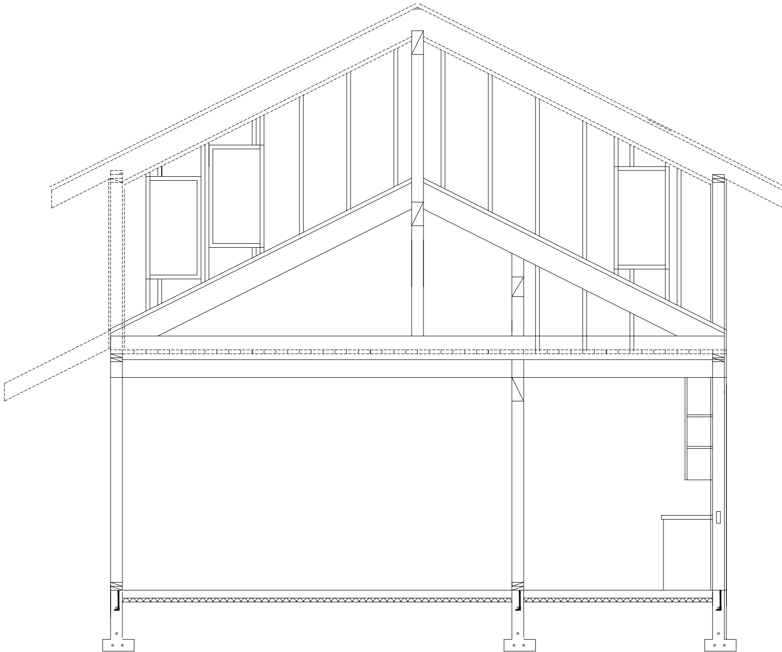
X-SECTION S-N-2
