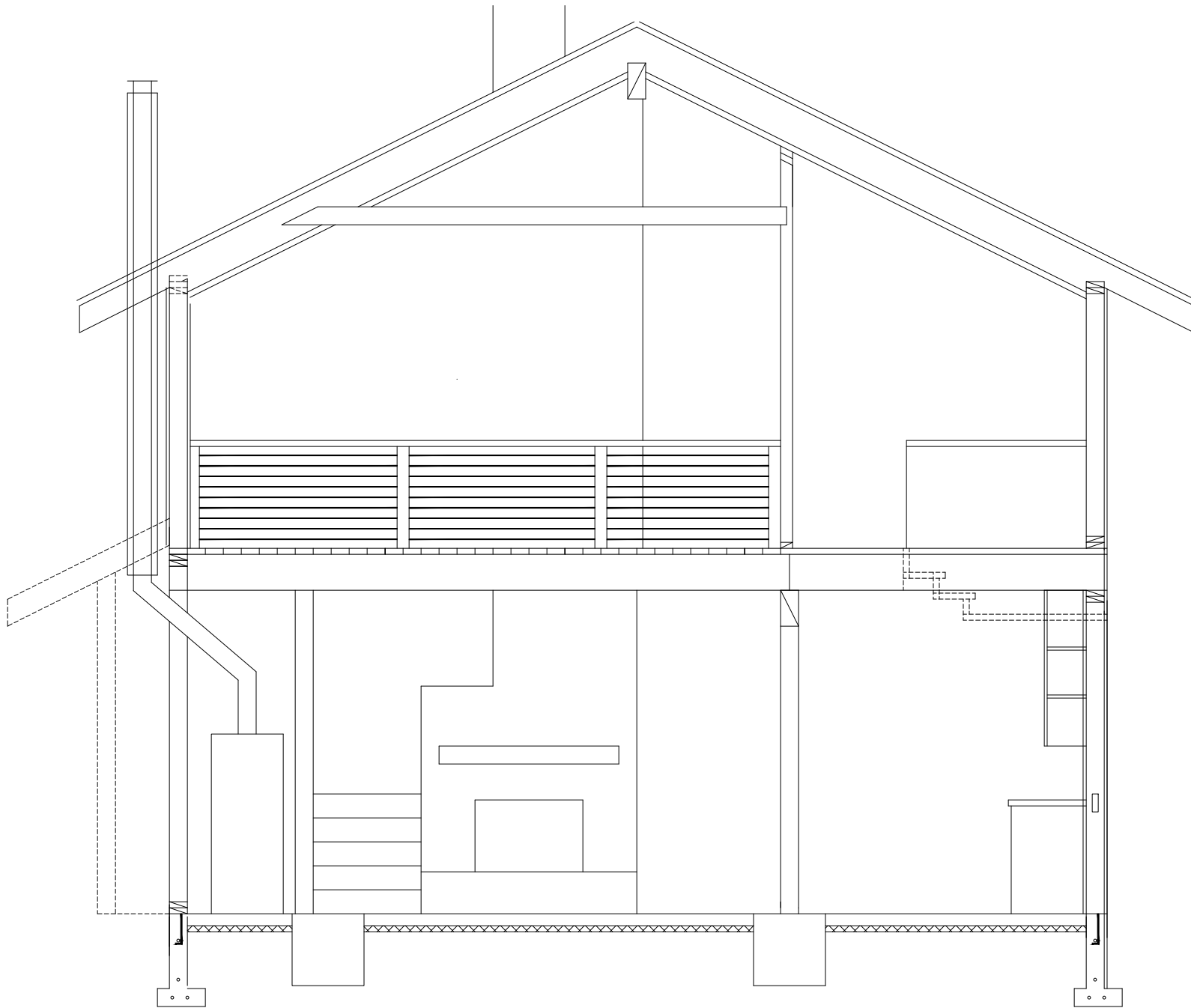
X-SECTION S-N-3
