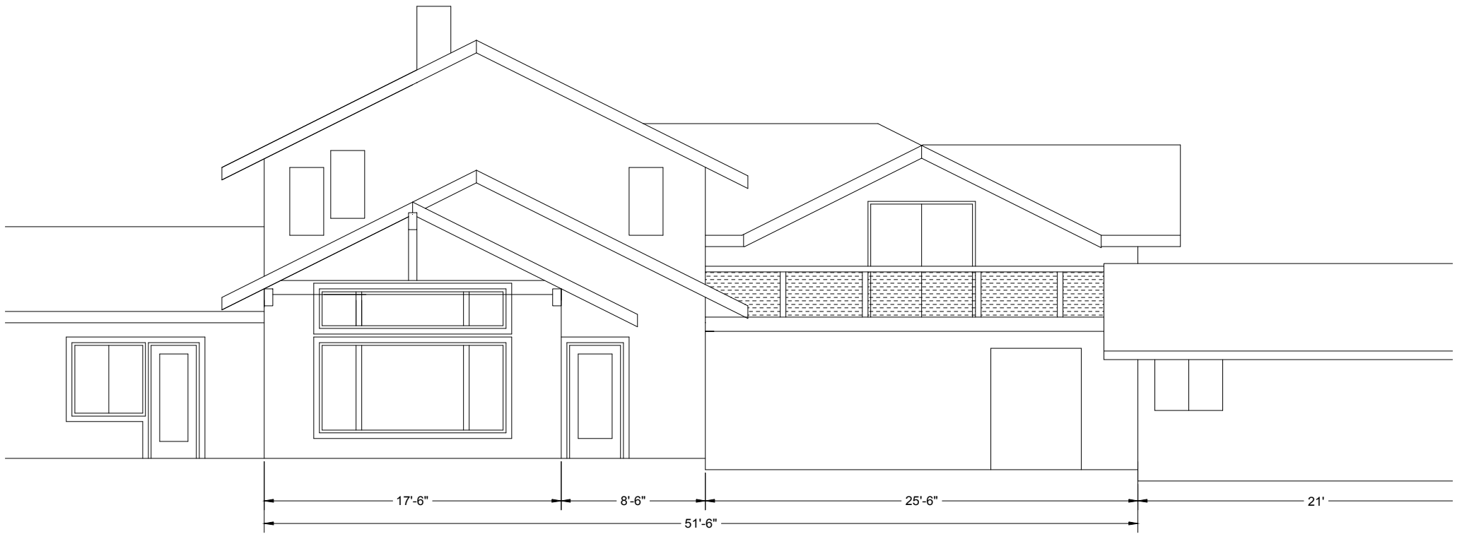
East Elevation
