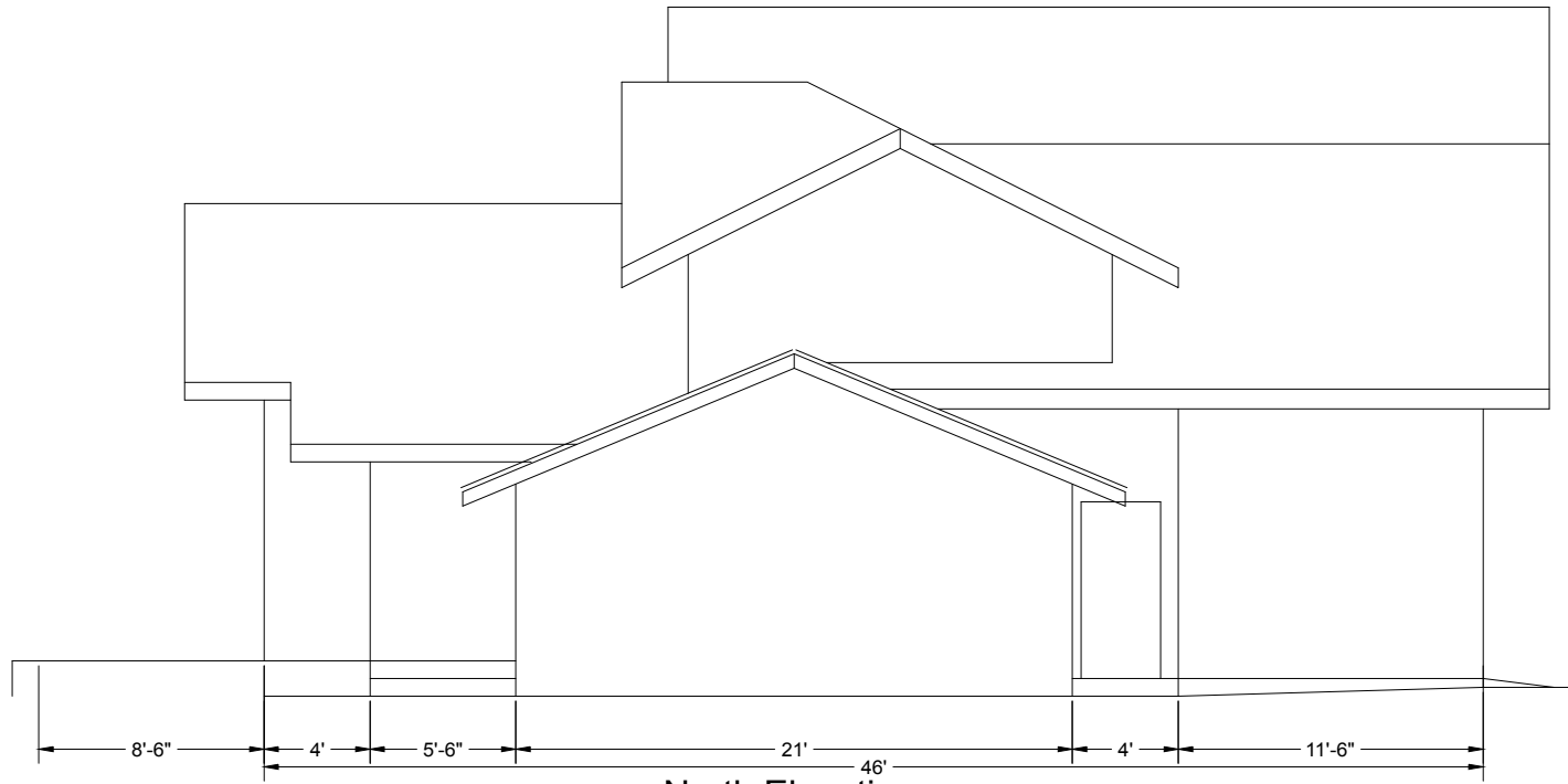
North Elevation
